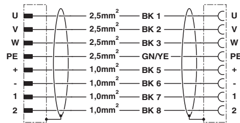
Contact assignment of M40 plugs/sockets
